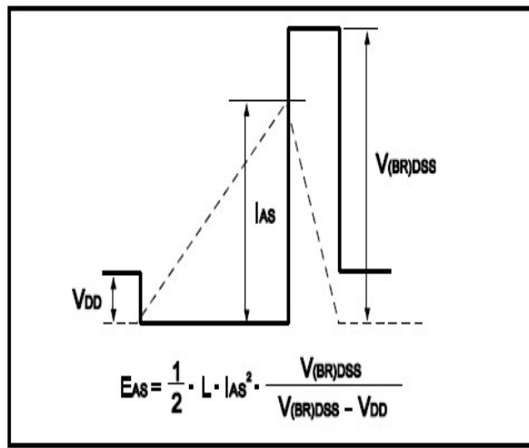
Fig.12 Avalanche Waveform
